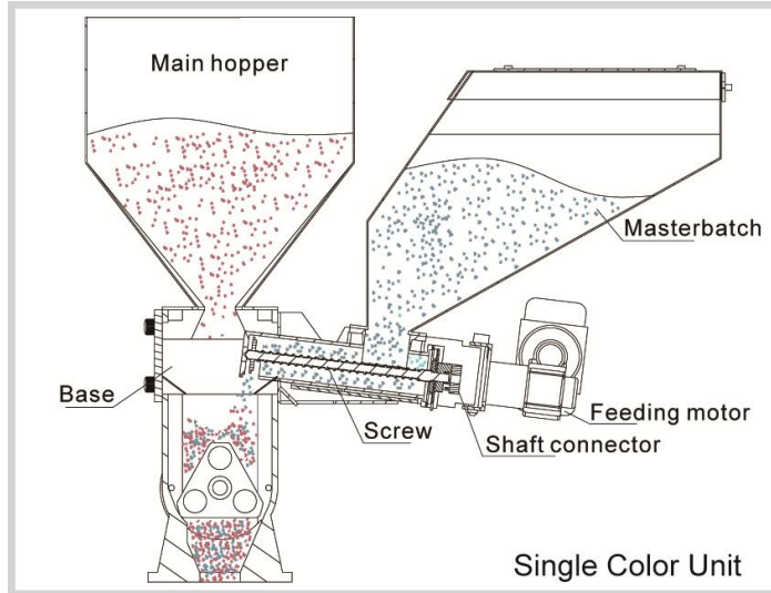
Picture 2-1: Working Principle
