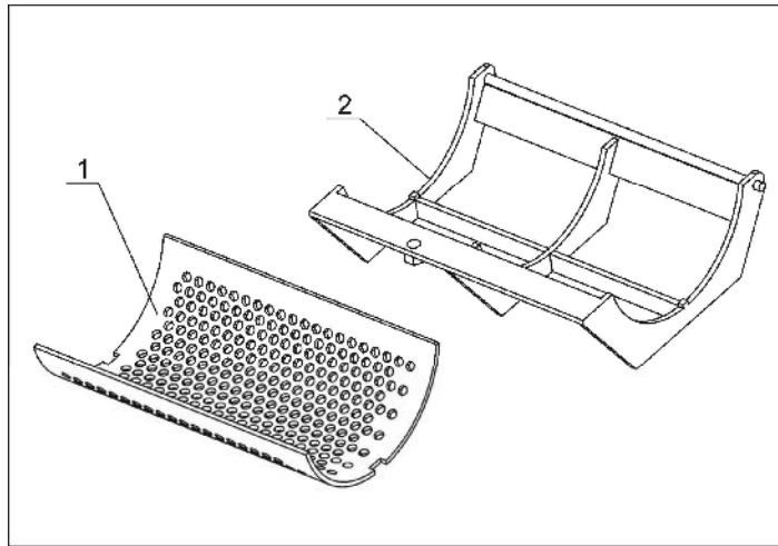
Picture 2-17: Screen and Screen Frame
