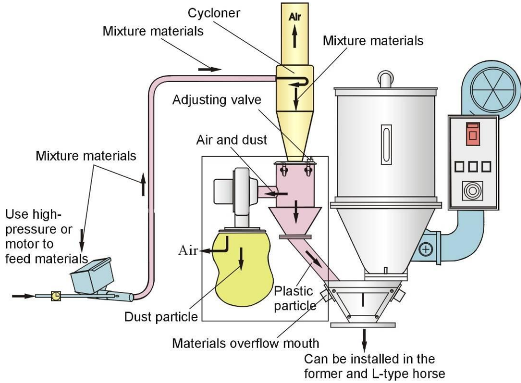
Picture 2-43: Dust separating System
