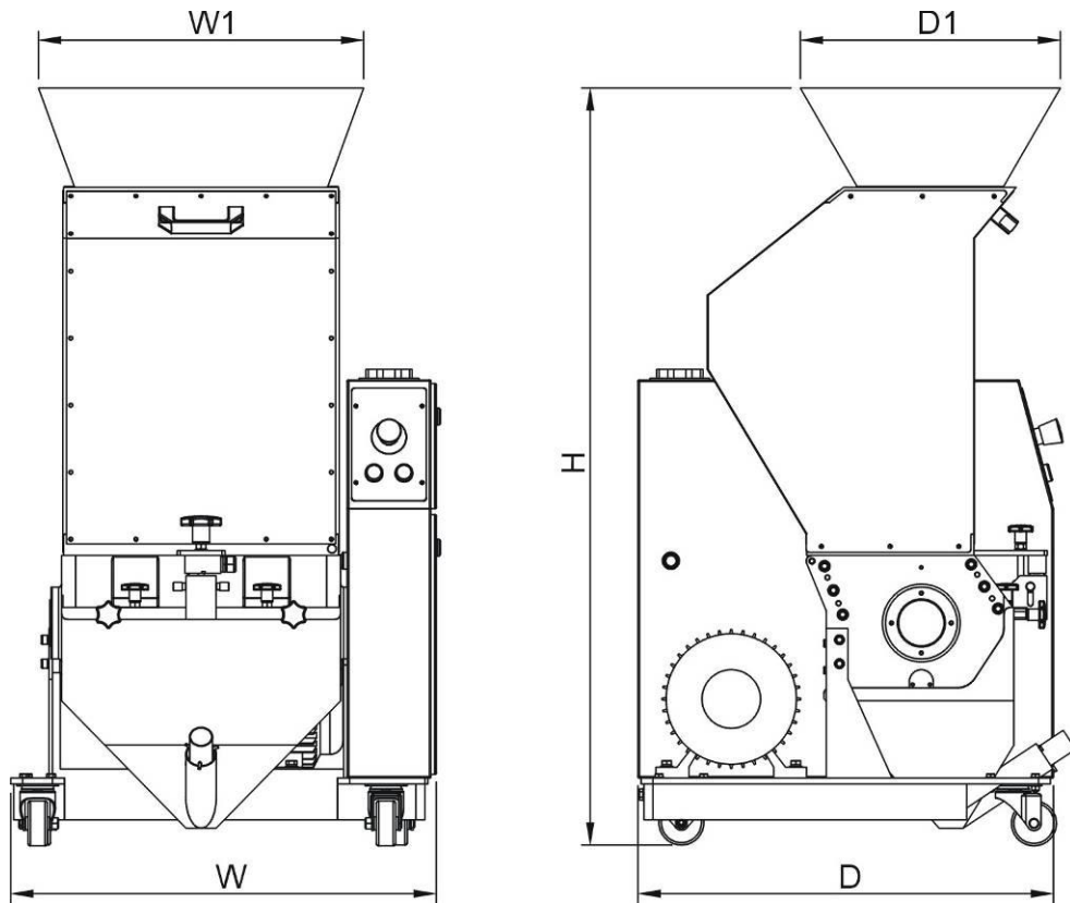
Picture 1-2: Dimensions (SG-20N)
