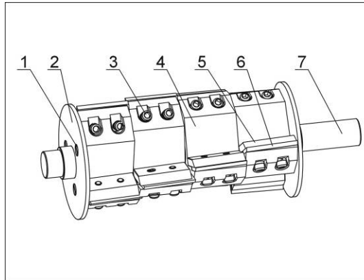
Picture 2-13: Unadjustable Staggered Blade
