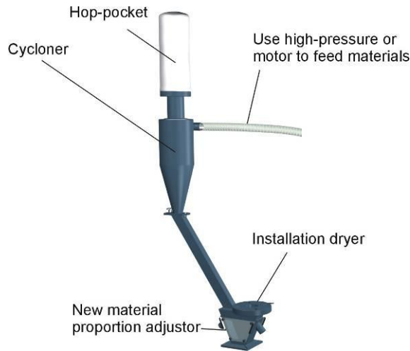
Picture 2-31: 30 Seconds Instant recycling system
