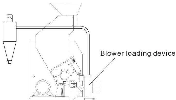
Picture 2-40: Option 3: Blower + Cyclonic Loading Device
