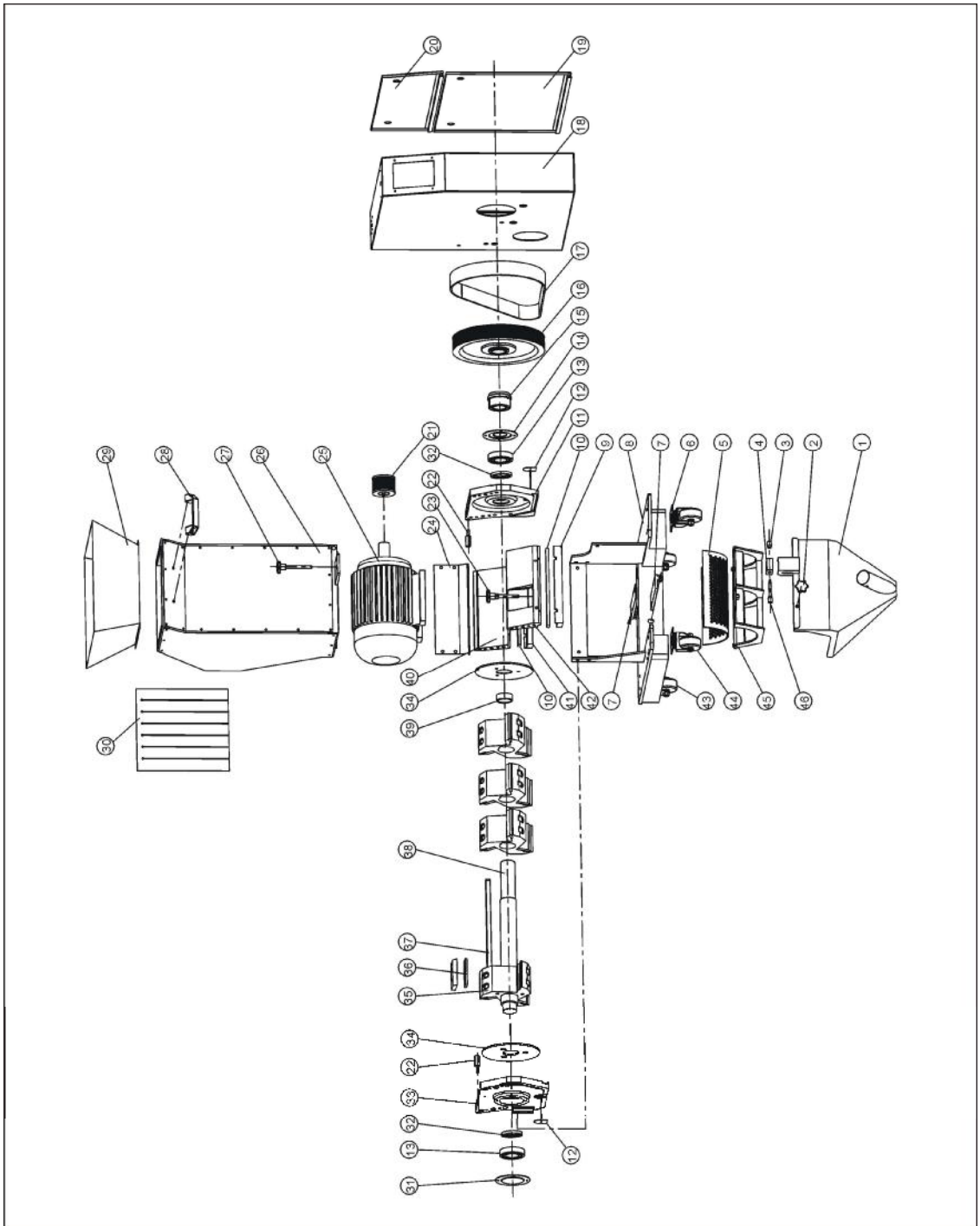
Picture 2-6: Assembly Drawing (SG-1628N(S))
