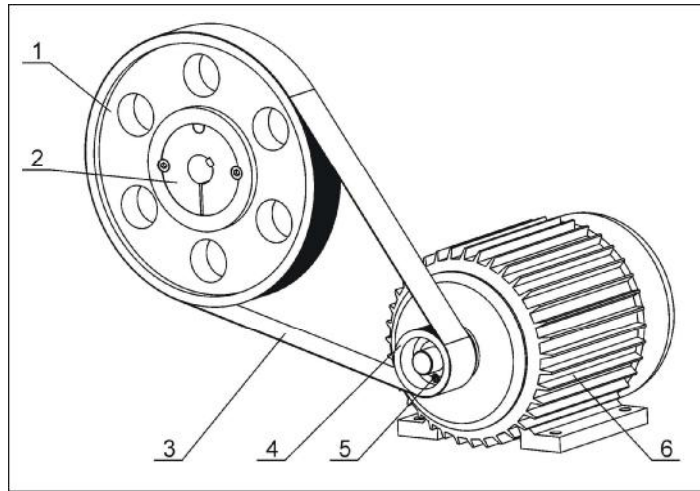
Picture 2-15: Transmission Parts
