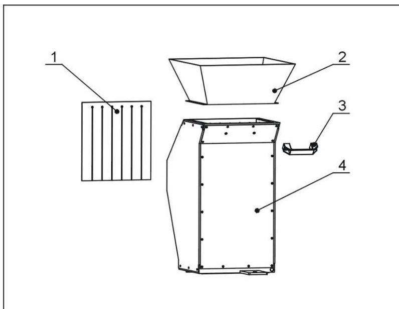
Picture 2-16: Feed Port, Feed Box and Material Check Plate
