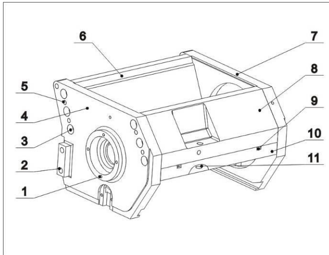
Picture 2-12: Cutting Chamber
