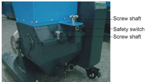
Picture 2-2: Safety System
