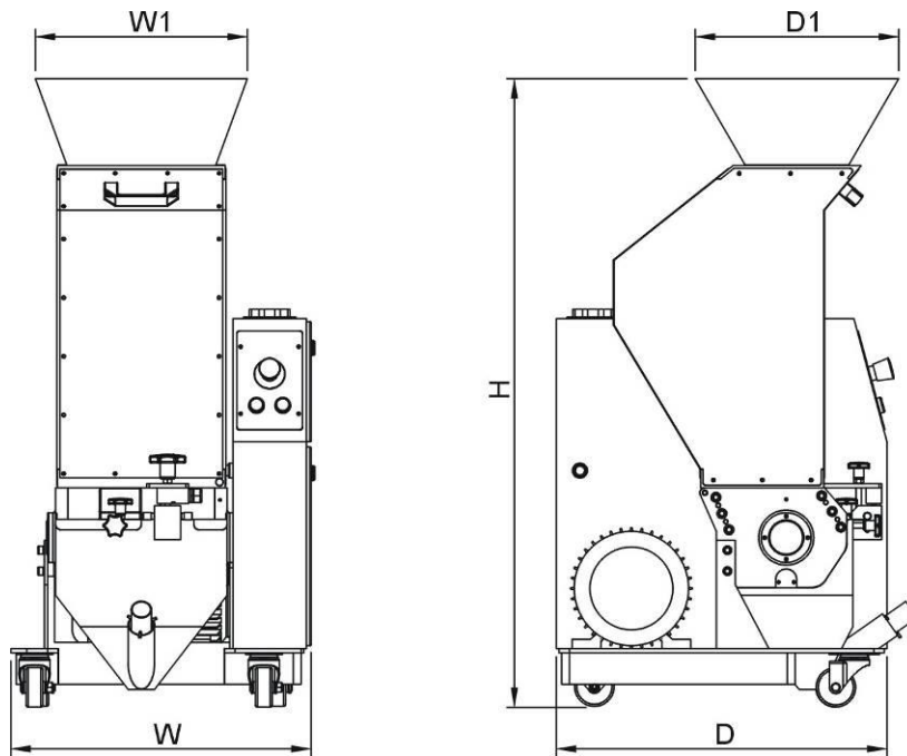
Picture 1-1: Dimensions (SG-16N)
