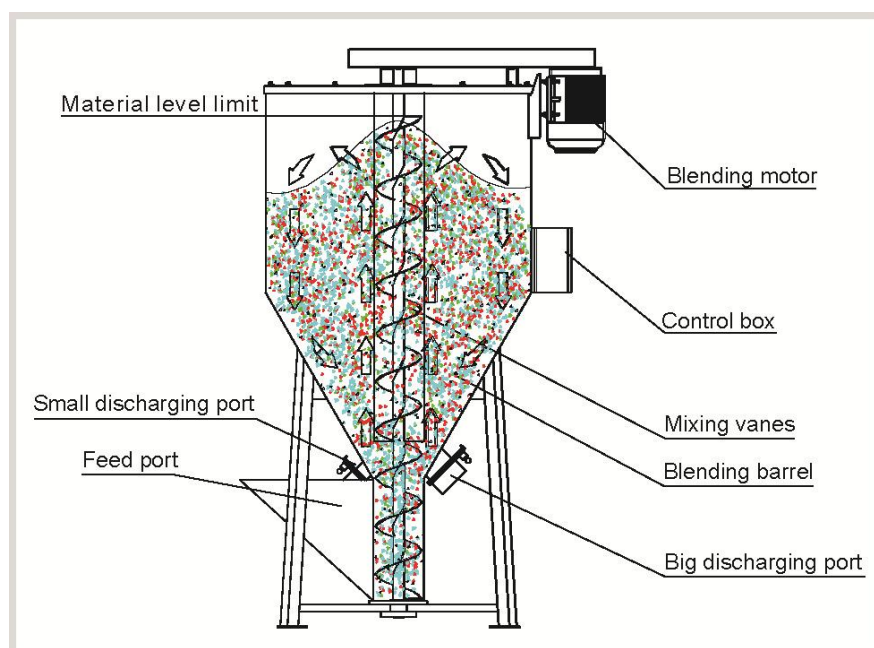
Picture 2-1: SVM-750U Working Principle Illustration
